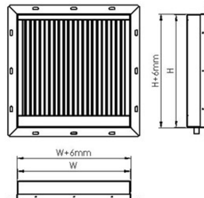
Drawing: CamVane AL WxHx100-DU FAR
